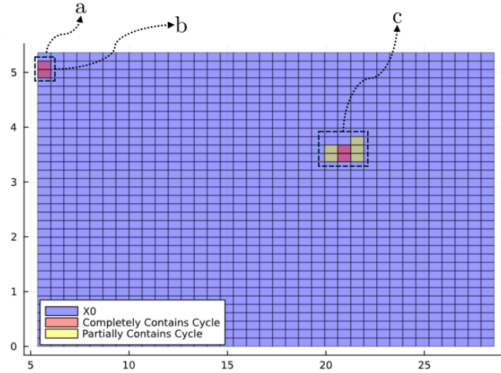
Figure 1: xy -projection of the cross-section, that maps onto itself, showing the geometric classification results. Region a ( small_X0[1191] ) contains the steady-state point and was excluded from the reachability analysis. Region b ( small_X0[1121, 1156] ) shows a false “Completely Contains Cycle” classification arising from convergence near the steady state. Region c ( small_X0[793:795, 828:830, 865] ) corresponds to the cluster of boxes through which the limit cycle passes completely or partially.
